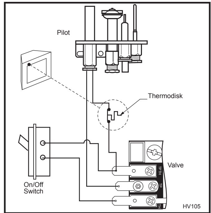
Fig. 11 Remote switch wiring.
