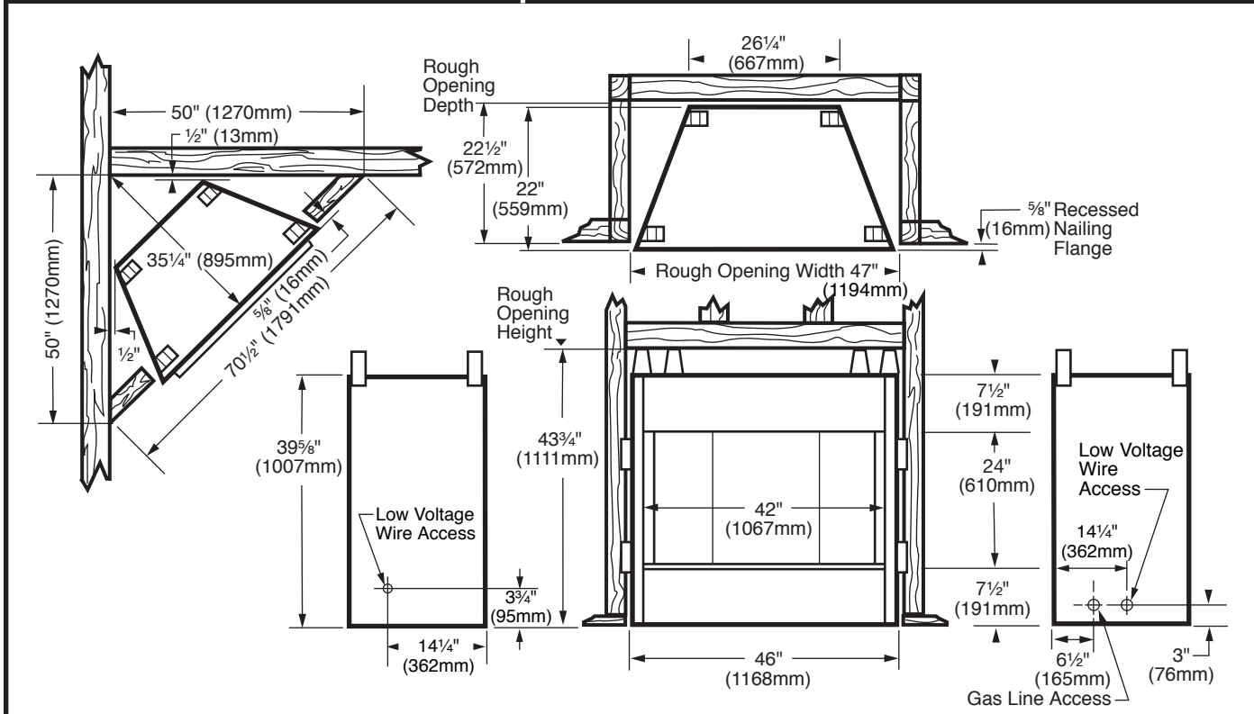
Fig. 2 ODGSR42A specification and framing dimensions.
