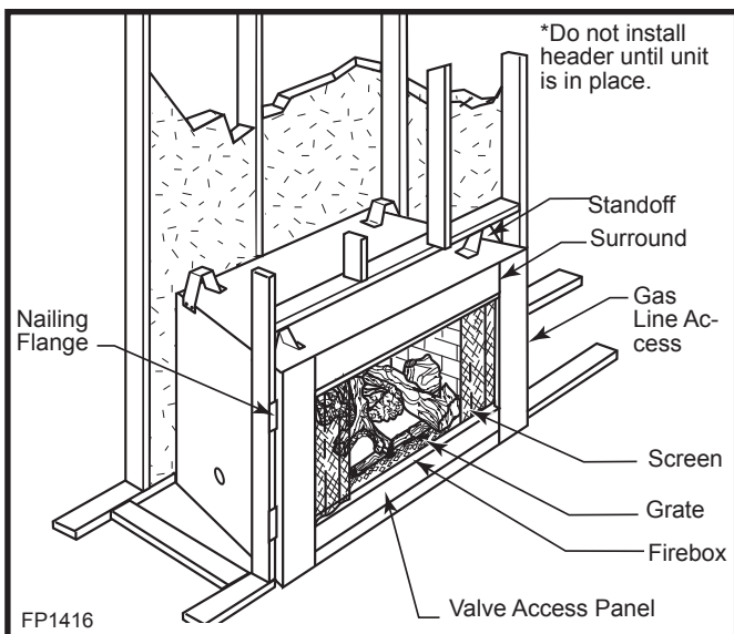
Fig. 8 Parts identification.
