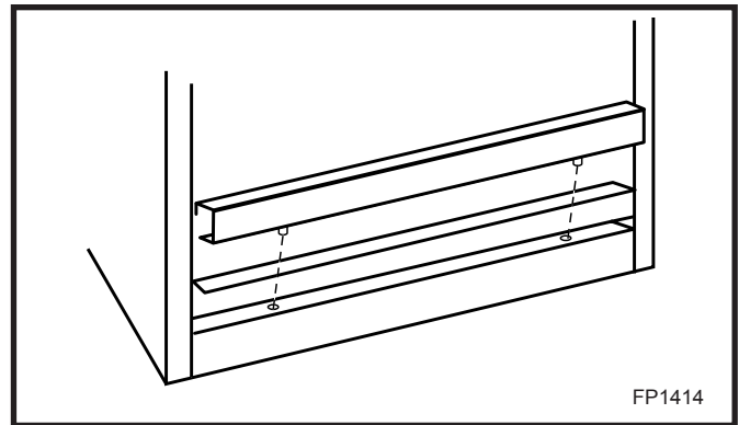
Fig. 5 Valve access.
