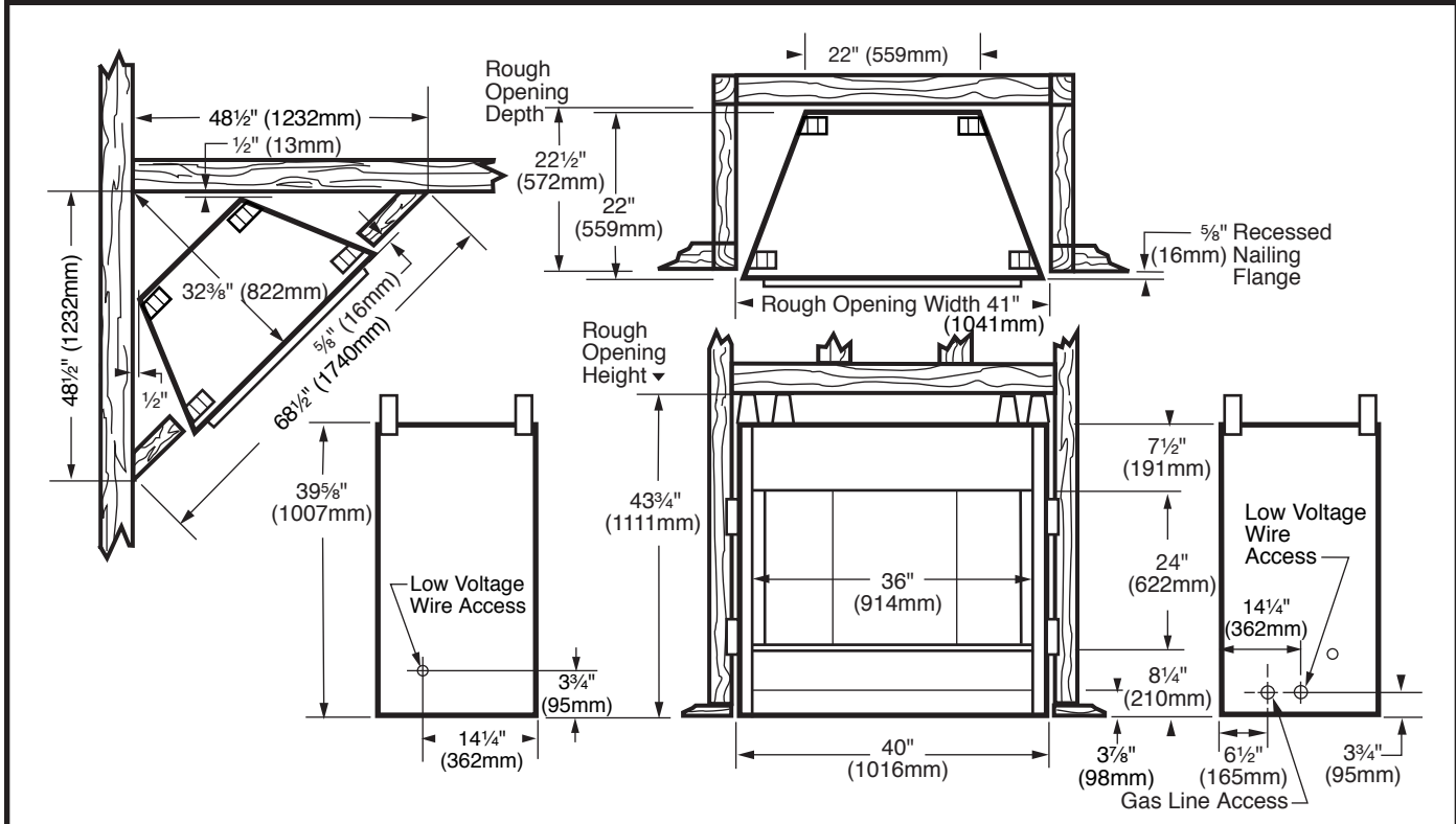
Fig. 1 ODGSR36A specification and framing dimensions.
